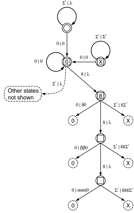
Figure 10. A portion of the graph of particle filter T_{54}^1 , which maps domain cells to 0, cells in the fundamental particles to output symbols \{\alpha, \beta, \gamma^+, \gamma^-\} and strings occurring in pairwise \alpha - \gamma interactions to \delta . All other defects are left changed, since they do not correspond to recognized structures. The input label \Sigma' denotes all input symbols not found on other edges leaving a given state. Edges terminating on broken circles actually reconnect to the indicated state at the top of the machine; they have been displayed in this way for clarity. Note that the number of output symbols in an edge label varies from zero (indicated by \lambda ) to four. Not shown are the other seven edges leaving state 0, corresponding to input symbols \{1, \dots, 7\} . Each of these edges leads to a different group of states and edges similar to the one shown.
