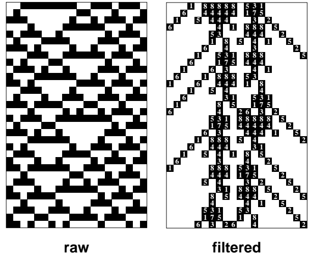
Figure 15. Raw (a) and filtered (b) space-time diagrams of the gamma gun. The gamma gun arises from the decay of the unstable domain shown in fig. 14(b).
