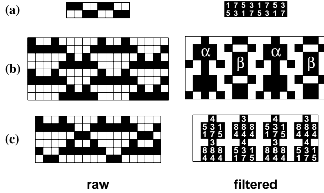
Figure 14. Unfiltered and filtered space-time diagrams of a few of ECA 54's other domains. (a) An unstable domain. (b) A domain consisting of alternating \alpha s and \beta s. (c) A domain of "pseudo- \alpha s" in which every block of nonzero filtered cells is either part of an \alpha or is a string occurring in an \alpha - \gamma interaction. In the filtered plots, domain cells are white, particles are black and non-particle defects are black with T_{54}^0 output symbol.
