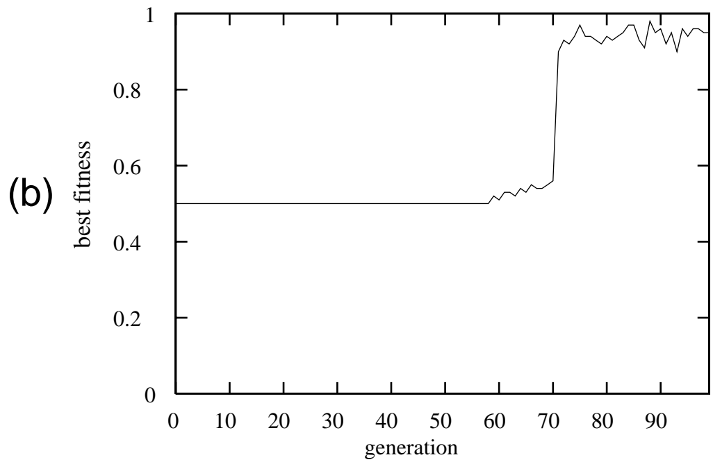
Figure 16: Best fitness versus generation for two of the 50 runs performed with no crossover.
