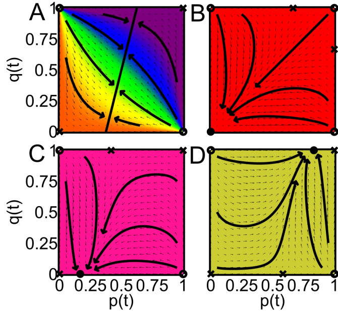
FIG. 2: Vector fields (small arrows), sample trajectories (large arrows) and phase diagrams (colored areas) for two interacting populations with incompatible preferences, playing snowdrift games with B > 0 and C < 0 (right). The representation is the same as in Fig. 1. In particular, the colored areas represent again the basins of attraction, i.e. all initial conditions (p(0), q(0)) leading to the same fix point [red = (0,0) , salmon = (u,0) , mustard = (v,1) , rainbow colors = (u,v) , with 0 < u, v < 1 ]. The model parameters are as follows: (A) |B| = |C| = 1 and f = 0.8 , i.e. 80% of all individuals belong to population 1, (B) |C| = 2|B| = 2 and f = 1/2 , i.e. both populations are equally strong, (C) |C| = 2|B| = 2 and f = 0.8 , (D) 2|C| = |B| = 2 and f = 0.8 . (A) In the multi-population snowdrift game (MSD), a mixture of cooperative and uncooperative behaviors results in both populations, if |B| = |C| . (B) For |B| < |C| and equally strong populations, everybody ends up with non-cooperative behavior in each population. (C) For |B| < |C| and f - 1/2 \gg 0 , the weaker population 2 solidarizes with the minority of the stronger population 1 and opposes its majority. (D) Same as (C), but now, all individuals in the weaker population 2 show their own preferred behavior after the occurrence of a discontinuous (“revolutionary”) transition of the evolutionary equilibrium from (u, 0) to (v, 1) .
