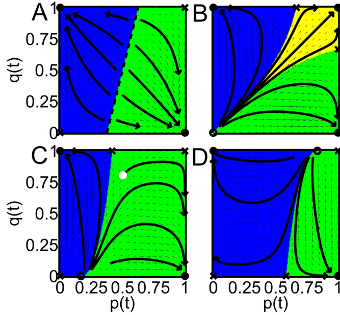
FIG. 1: Vector fields (small arrows), sample trajectories (large arrows) and phase diagrams (colored areas) for two interacting populations with incompatible preferences, playing stag hunt games with B < 0 and C > 0 (right). p is the fraction of individuals in population 1 showing their preferred, cooperative behavior 1, and q is the fraction of cooperative individuals in population 2 showing their preferred behavior 2. The vector fields show (dp/dt, dq/dt) , i.e. the direction and size of the expected temporal change of the behavioral distribution, if the fractions of cooperative individuals in populations 1 and 2 are p(t) and q(t) . Sample trajectories illustrate some representative flow lines (p(t), q(t)) as time t passes. The flow lines move away from unstable stationary points (empty circles or dashed lines) and are attracted towards stable stationary points (black circles or solid diagonal lines). The colored areas represent the basins of attraction, i.e. all initial conditions (p(0), q(0)) leading to the same fix point [yellow = (1,1) , blue = (0,1) , green = (1,0) ]. Saddle points (crosses) are attractive in one direction, but repulsive in another. The model parameters are as follows: (A) |B| = |C| = 1 and f = 0.8 , i.e. 80% of all individuals belong to population 1, (B) |C| = 2|B| = 2 and f = 1/2 , i.e. both populations are equally strong, (C) |C| = 2|B| = 2 and f = 0.8 , (D) 2|C| = |B| = 2 and f = 0.8 . In the multi-population stag hunt game (MSH), due to the asymptotically stable fix points at (1,0) and (0,1) , all individuals of both populations finally show the behavior preferred in population 1 (when starting in the green area) or the behavior preferred in population 2 (when starting in the blue area). This case can be considered to describe the evolution of a shared behavioral norm. Only for similarly strong populations ( f \approx 1/2 ) and similar initial fractions p(0) and q(0) of cooperators in both populations (yellow area), both populations will end up with population-specific norms (“subcultures”), corresponding to the asymptotically stable point at (1,1) . The route towards the establishment of a shared norm may be quite unexpected, as the flow line starting with the white circle shows: The fraction q(t) of individuals in population 2 who are uncooperative from the viewpoint of population 1 grows in the beginning, but later on it goes down dramatically. Therefore, a momentary trend does not allow to easily predict the final outcome of the struggle between two interest groups.
