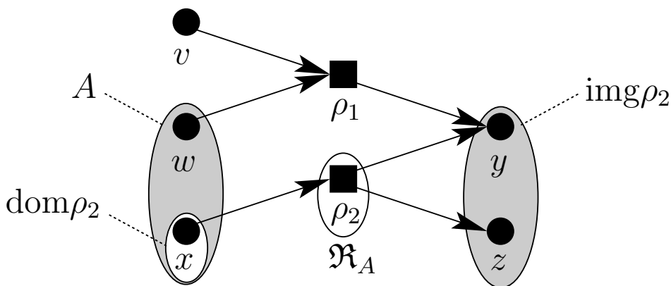
Fig. 2. If only a subset A of all chemical species X is present in the reaction mixture, then only those reactions can take place whose educts \text{dom}\rho_i are elements of A . This is only true for \rho_2 in the shown reaction network.
