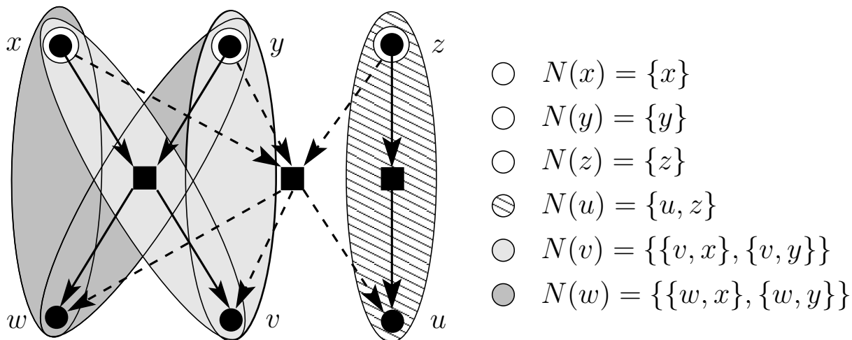
Fig. 7. Minimal neighborhoods for each of the species i \in \{x, y, z, u, v, w\} in a reaction network composed of two “elementary” reactions (bold arrows) and a super-reaction (dashed arrows) which performs the same chemical transformation as the superposition of the two elementary reactions. By definition, all supersets of neighborhoods are also neighborhoods. In contrast to graphs, the minimal neighborhoods are not unique. For instance, w has the two minimal neighborhoods \{w, x\} and \{w, y\} .
