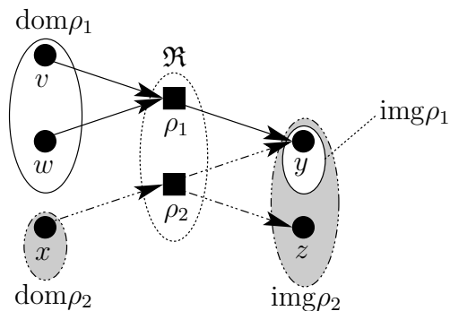
Fig. 1. Illustration of the chemical universe (X, \mathfrak{R}) for the chemical reaction network composed of the two reactions \rho_1 : v + w \rightarrow y and \rho_2 : x \rightarrow y + z . The chemical universe is the tuple of the set of species X = \{v, w, x, y, z\} and the set of chemical reactions \mathfrak{R} = \{\rho_1, \rho_2\} .
