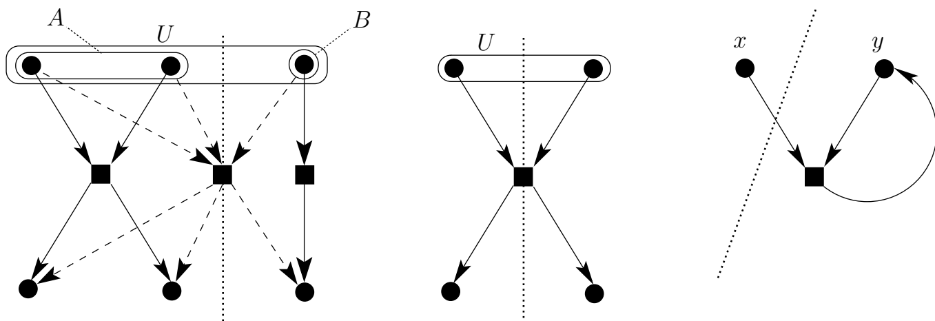
Fig. 8. Illustration of the concepts separated, semiseparated and productively connected. (Left chart) The reaction network is separated although from a graph theoretical view point, the network is connected. This classification makes sense since in a chemical sense nothing new is gained by the super-reaction (dashed arrows) which holds the network together in the sense of graph theory. (Middle chart) The reaction network is semi-separated. (Right chart) The reaction network is productively connected with respect to p' since something new is produced from the union of the subsets ( p'(\{x\}) = p'(\{y\}) = p'(\{x\}) \cup p'(\{y\}) = \emptyset and p'(\{x\} \cup \{y\}) = \{y\} ). With respect to p the reaction network is not productively connected because nothing new can be produced that was not already part of one of the two subsets ( p(\{x\}) = \{x\} , p(\{y\}) = \{y\} and p(\{x\}) \cup p(\{y\}) = p(\{x\} \cup \{y\}) = \{x, y\} ).
