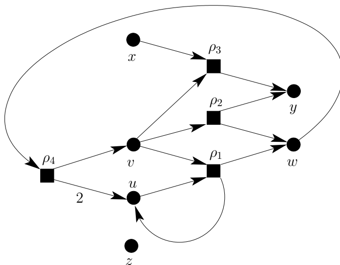
Fig. 6. Illustration of the set-valued set-functions m , s , and s^* for the set A = \{u, v, w, x, y, z\} . The reaction network is essentially the one from Fig 5. with the additional reaction \rho_4 . The species x and v are not maintainable. The set of self-maintaining chemical species is m(A) = \{u, w, y, z\} . If outflow is applied to the produced species in the set A , the set of maintainable species is reduced to the set of stationary produced species s(A) = \{u\} . If outflow is applied to all species in A , the set of stationary produced species is reduced to s^* , which in this case is the empty set.
