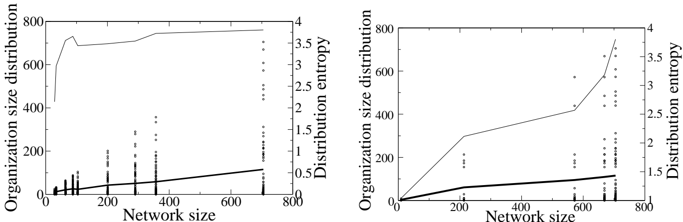
Fig. 4. Change of the set of organizations in a growing network. Network size increases by increasing the number of allowed molecules (left chart), or the number of starting molecules (right chart). For each network size, the sizes of all organizations form a distribution ( \circ ) which is shown with its mean (connected by the bold black line) and its entropy (connected by a black line).
