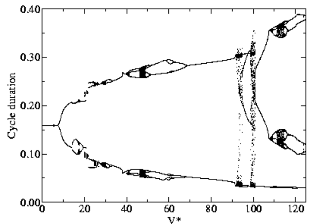
FIG. 5: Dependence of the replication time on the monomers threshold for the case of strong replication condition with N = 10 and \bar{X} = 10 .
