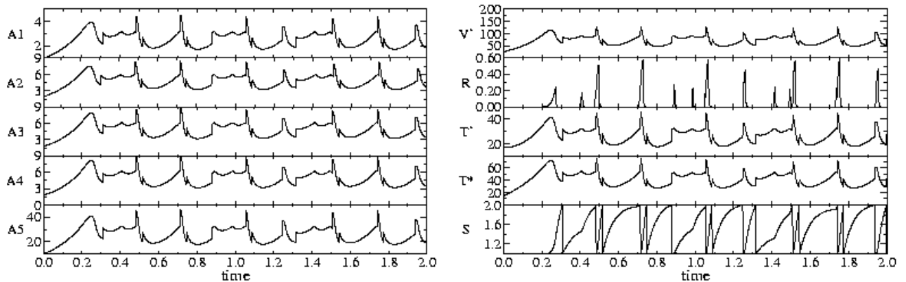
FIG. 6: Time series of metabolites concentration for the strong condition of template replication: \bar{X} = 100 , N = 10 , V^* = 90 . This case is representative for a dynamics characterized by a diversity of self-replication periods. See Fig. 4.
