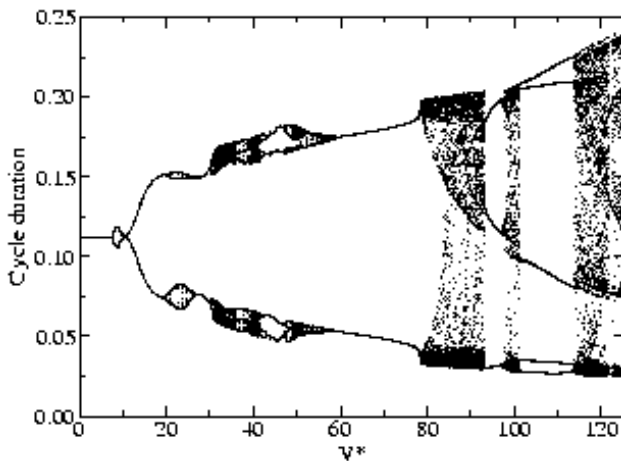
FIG. 4: Dependence of the replication time on the monomers threshold for the case of strong replication condition with N = 10 and \bar{X} = 100 .
