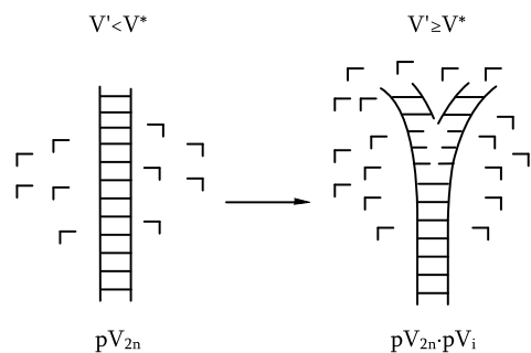
FIG. 1: Template chains may open randomly and for monomers' concentration V' below the critical threshold V^* , the opposite ends reconnect. For V' \geq V^* , bonding with available monomers can occur, leading to the zip-like replication of the polymer pV_{2n} .
