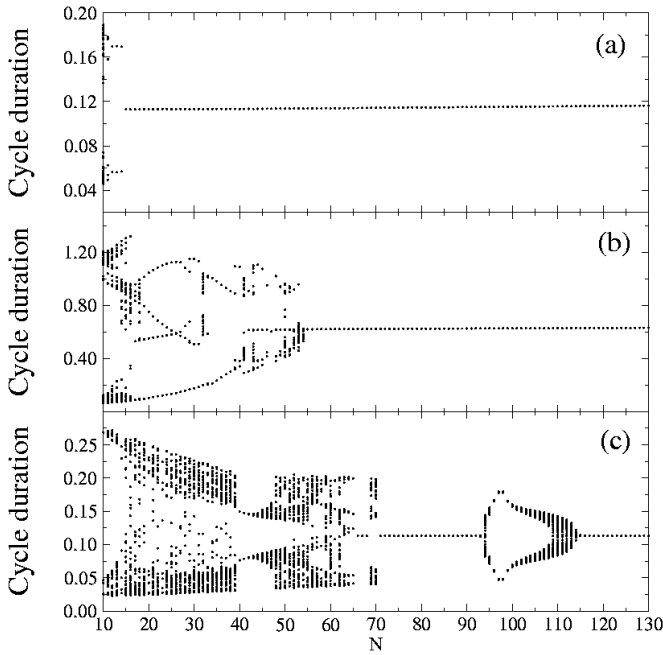
FIG. 9: Dependence of the replication time on the template length for the weak replication condition for the cases of (a) X = 100 , V^* = 35 and k_7 = 10 ; (b) X = 1 , V^* = 35 and k_7 = 10 ; (c) X = 100 , V^* = 35 and k_7 = 100 .
