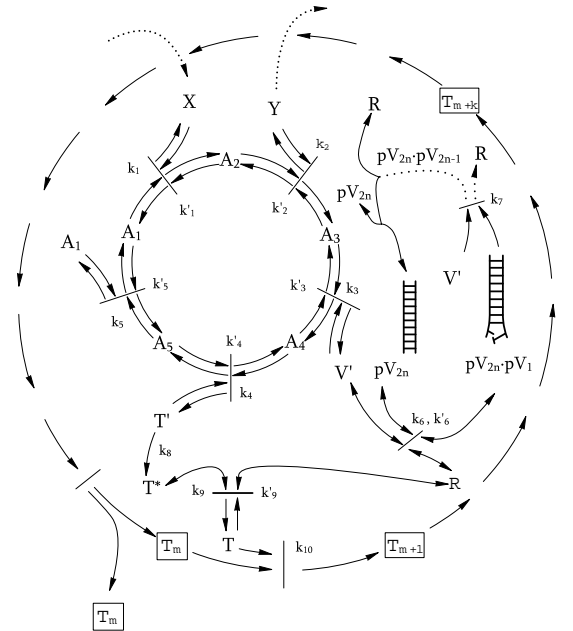
FIG. 2: The chemoton: the metabolic unit, the template (information) subunit and the membrane subsystem. The dots in the template subsystem indicate the iterative development of the template replication from pV_{2n} \cdot pV_1 to pV_{2n} \cdot pV_{2n-1} .
