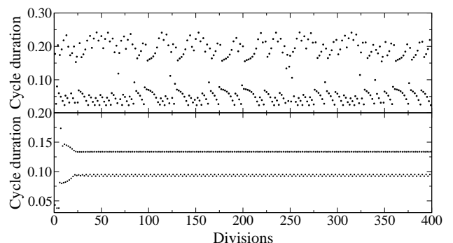
FIG. 8: Temporal evolution of the replication period for N = 10 , \bar{X} = 100 : (upper panel) V^* = 100 and (lower panel) V^* = 55 . See Fig. 7.
