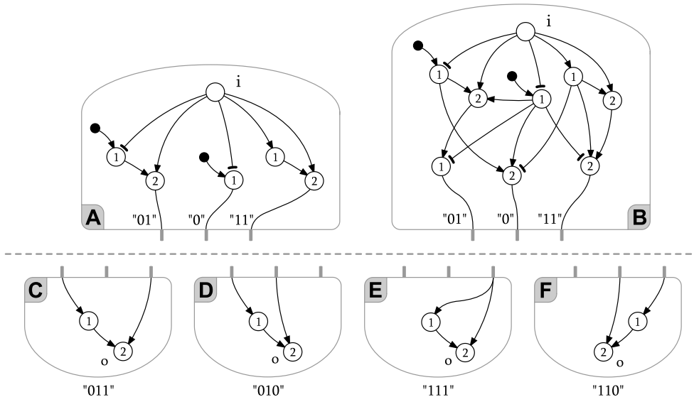
FIG. 8: An example of modularity in Boolean networks. A Module that makes useful “pre-detections”. B The same module with added robustness. C, D, E & F. Various ways to use the basic module to perform different functions.
