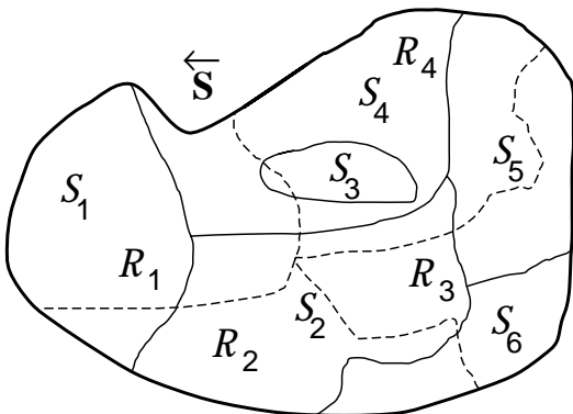
FIG. 2. An alternative class \mathcal{R} of states (delineated by dashed lines) that partition \overleftarrow{S} overlaid on the causal states \mathcal{S} (solid lines). Here, for example, S_2 contains parts of \mathcal{R}_1 , \mathcal{R}_2 , \mathcal{R}_3 and \mathcal{R}_4 . Note again that the \mathcal{R}_i need not be compact nor simply connected, as drawn.
